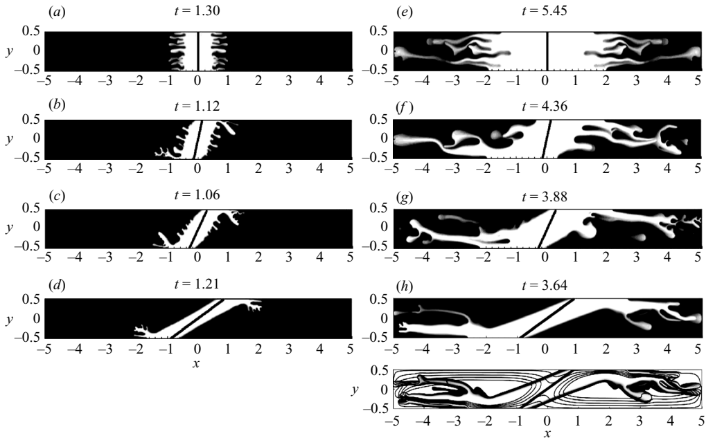
FIGURE 13. Displacement fronts for R = 3 , G = 0 , Pe = 2000 and \alpha = 0^\circ, 15^\circ, 30^\circ and 60^\circ , respectively. Similarly to lower mobility ratios, a single dominant finger quickly forms for each inclined front. However, in contrast to lower mobility ratio displacements, this dominant finger separates from the reservoir boundary and propagates towards the reservoir centreline, while undergoing repeated splitting events.
