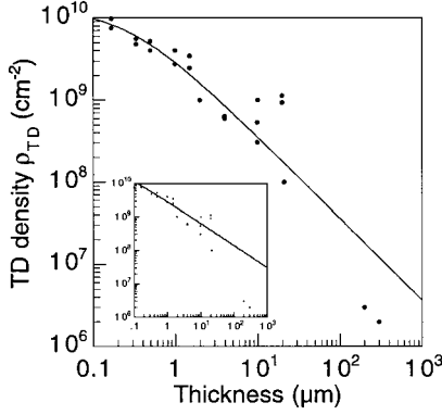
Fig. 9. Experimental GaN dislocation density data. The data from [11] were fitted with Eq. (2), giving a value for K \approx 275 \text{ \AA} , and K \approx r_A . The inset shows the experimental behavior compared to a 1/h^{2/3} fit. When the experimental data are not weighted, an exponent n = 0.66 is found (for \rho_{TD} \propto 1/h^n )
