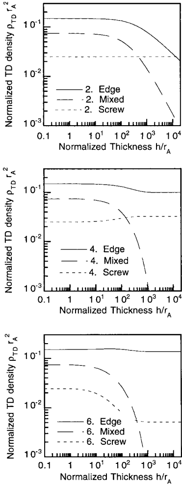
Fig. 6. Subdensity comparison for cases 2, 4 and 6, each having 60% edge, 30% mixed, and 10% screw dislocation densities initially. a) Case 2: Screw dislocations, which were not allowed to react, have a constant density. Edge and mixed TD densities decrease without saturating. b) Case 4: Screw TDs are allowed to react, and their density increases, then saturates with thickness. The edge dislocation density also saturates. This saturation happens at a thickness corresponding to the point when the mixed TD density falls suddenly, or when the mixed TDs are depleted. c) Case 6: Screw TDs are 10 times as reactive as in case 4. The screw and edge TD density both decrease with thickness, but saturate when mixed TDs are depleted. This happens at a smaller thickness and a larger TD density
