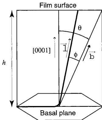
Fig. 3. Angles used in the calculation of line direction. \phi is the angle between the Burgers vector and line direction. \theta is the angle between the Burgers vector and [0001] , which is the shortest possible line direction for GaN dislocations in (0001) film growth
