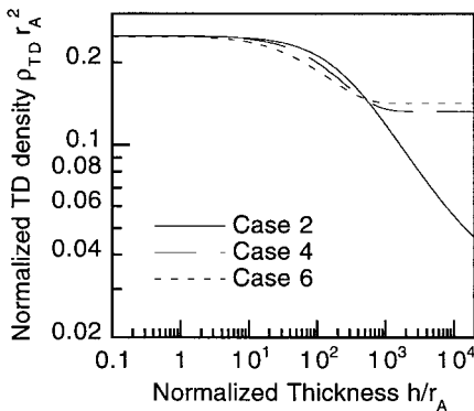
Fig. 5. TD density falloff for cases 2, 4 and 6. Case 2, with 60% edge, 30% mixed, and 10% screw dislocations, but no allowed screw dislocation reactions, results in no TD density saturation. Cases 4 and 6, with the same initial TD subdensities, had screw reactions allowed. Case 4, with normal screw TD reactivity ( r_A and K_{ij} ), saturated at a lower TD density than case 6, which had a high screw reactivity ( r_A and K_{ij} were an order of magnitude larger)
