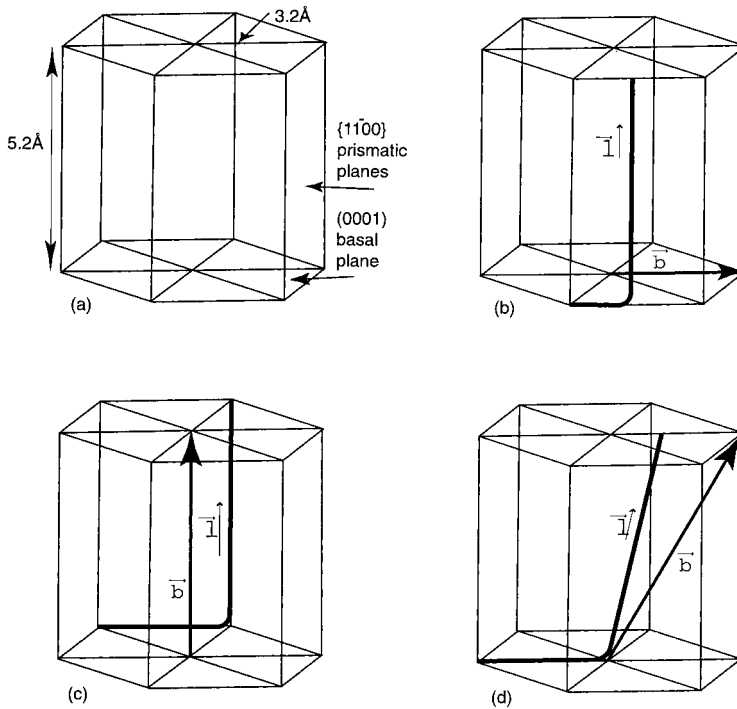
Fig. 1. GaN crystallography. a) The GaN unit cell has c = 1.62a . b) Edge dislocations in GaN with Burgers vectors of the type \langle 11\bar{2}0 \rangle and a vertical line direction. c) Perfect screw dislocations with \mathbf{b} = \pm[0001] and line direction [0001] . d) Mixed character dislocations with Burgers vectors of the type \langle 11\bar{2}1 \rangle and inclined line directions
