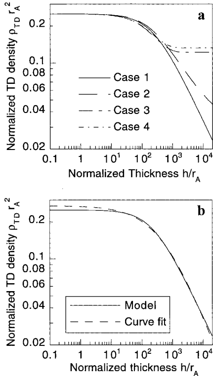
Fig. 4. Total TD density evolution with film thickness for cases 1 to 4. a) Cases 1 and 2, with no screw dislocation reactions allowed, do not display saturation behavior. Cases 3 and 4, with screw dislocation reactions allowed, reach a minimum TD density and saturate. Case 2, with an initial screw TD subdensity of 10% of the total TD density, has a higher final TD density than that of case 1, which had no screw TDs. Similarly, case 4, with an initial nonzero screw subdensity, saturated at a higher TD density than case 3. The maximum thickness corresponds to 250 \mu\text{m} for an annihilation radius of r_A = 500 \text{ \AA} . b) A curve fit of case 1 shows that the TD density depends on 1/h^{2/3} for large h . The best fit was found with \rho_{TD} r_A^2 = 1/[0.057(h/r_A)^{2/3} + 3.70]
