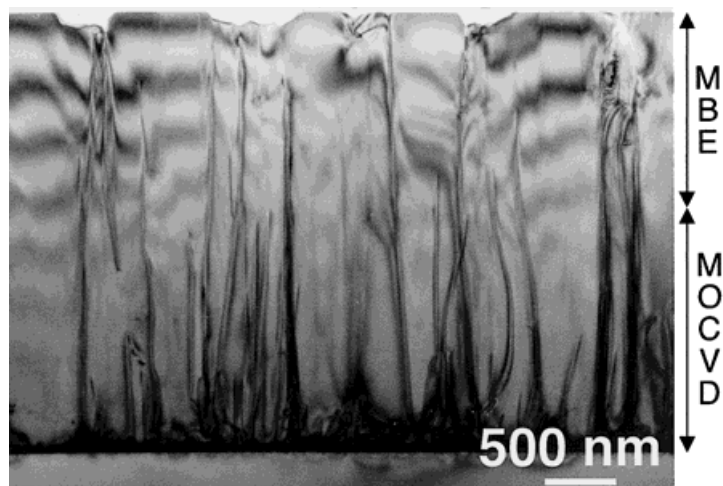
Fig. 2. Cross-section TEM micrograph of 1.4 \mu\text{m} MBE-grown GaN on a 1.6 \mu\text{m} MOCVD-grown GaN buffer. The micrograph is taken under \mathbf{g} = 0002 imaging condition. Under this imaging condition, only dislocations with a c -component Burgers vector are visible. Due to the low screw TD density, the dislocations are predominantly of mixed screw-edge character with line direction inclined at \approx 12.2^\circ to the surface normal. This angle was determined by taking the maximum inclination angle at sufficient distance from the film/substrate interface so that TD generation conditions did not dictate line direction. The maximum inclination was used because TDs lying in the plane normal to the viewing direction would have the largest apparent inclination, while those aligned with the viewing direction or at an angle < 90^\circ would have a smaller apparent inclination.
