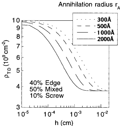
Fig. 8. The effect of annihilation radius on total TD density. Total TD density evolution for r_A values of 300 \text{ \AA} , 500 \text{ \AA} , 1000 \text{ \AA} , and 2000 \text{ \AA} . Screw dislocations reactions were allowed, resulting in saturation of the total TD density. Saturation happens at higher thicknesses for lower annihilation radii due to slower reactions between TDs, but the TD density at saturation is the same for the constant initial TD density of 10^{10}/\text{cm}^2 and equal initial subdensities
