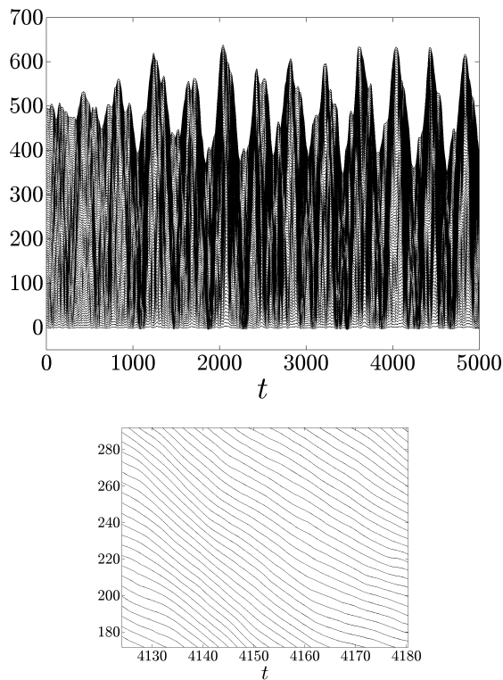
Fig. 1. Vehicle position trajectories (relative to leader) of a 100 vehicle formation all of which are subjected to random disturbances. Top graph is a “zoomed out” view exhibiting the slow accordion-like motion of the entire formation. Bottom graph is a zoomed in view showing that vehicle-to-vehicle distances are relatively well regulated.
